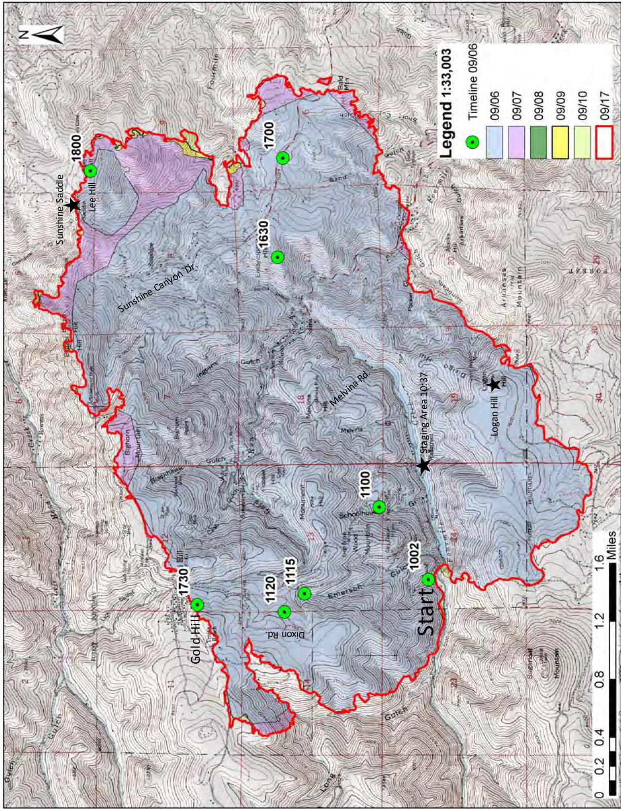
Figure 29. Daily progression of the Fourmile Canyon Fire. The points show the documented fire arrival times on September 6.
